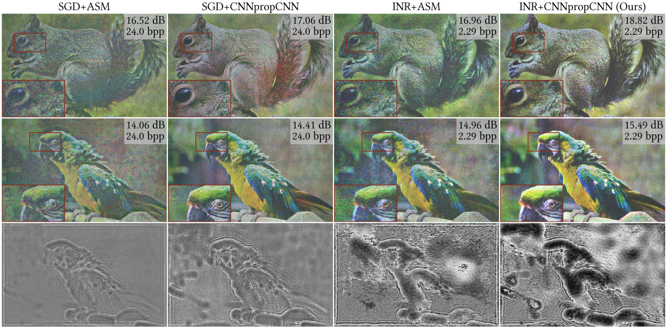
Fig. 6: Experimental reconstructions of 2D images using various CGH pipelines: SGD w/ ASM propagation, SGD w/ CNNpropCNN, INR w/ ASM, and INR w/ CNNpropCNN. This figure ablates the phase representation (SGD vs. INR) and the propagation model used during optimization (ASM vs. CNNpropCNN); the final configuration is INR w/ CNNpropCNN. All results are captured without a 4f system, akin to all other results in this manuscript. We present the achieved PSNR in dB and compression rates in bpp at their corners, as well as their corresponding phase-only holograms (green channel-only) for the second row example to display below.
