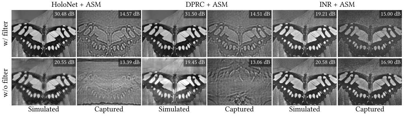
Fig. 10: Qualitative comparison for neural network-based CGH methods, including HoloNet, DPRC w/o compression, and our INR-CGH, each evaluated under two conditions: phase-only holograms generated with (top) and without (bottom) a Fourier aperture filter in simulation using ASM propagation. Within each group, the left column shows simulated reconstructions, while the right shows real captures with the same laser power and exposure time without a conventional 4f system, directly representing an unfiltered, compact display setup. Accordingly, the “with filter” simulation represents a reference configured with conventional Fourier aperture filtering. Note, we present green-channel acquisitions and visualize them as grayscale images.
