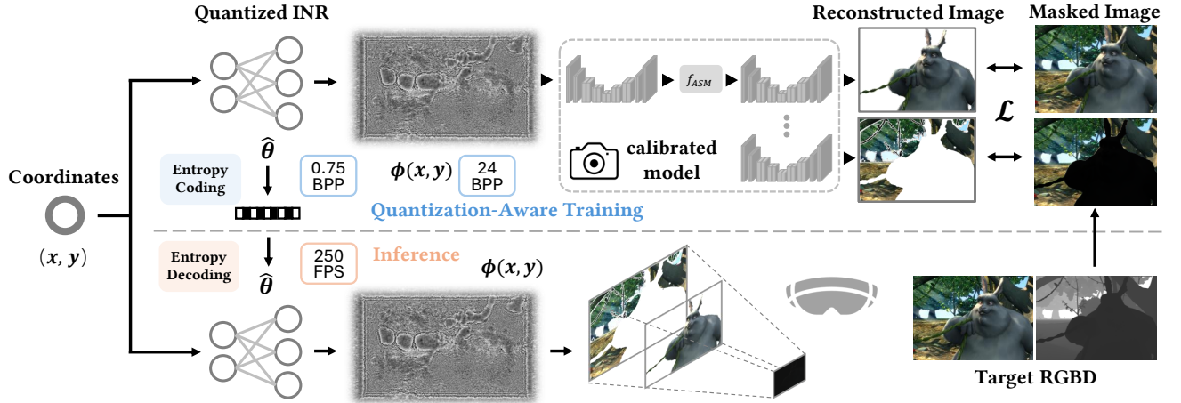
Fig. 2: Pipeline overview of our proposed INR-based hologram generation and compression, dubbed INR-CGH for brevity. On the server side, coordinates are input to the INR model, producing a compact and continuous representation of a phase-only hologram optimized through quantization-aware training with a camera-calibrated, learned propagation model and the RGBD supervision. INR parameters are subsequently compressed through quantization and entropy coding for efficient transmission. On the edge side, the compressed INR parameters are decoded and loaded, enabling rapid direct inference of phase-only holograms, which are then displayed on the spatial light modulator (SLM) for high-fidelity, unfiltered 3D reconstruction.
