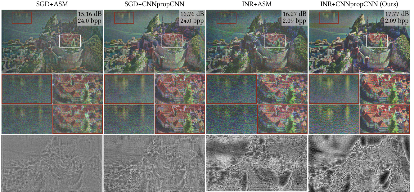
Fig. 7: Experimental reconstructions of 3D (RGBD) scenes using various CGH pipelines: SGD w/ ASM propagation, SGD w/ CNNpropCNN, INR w/ ASM, and INR w/ CNNpropCNN. We perform the same ablation in a 3D setting, varying the phase representation (SGD vs. INR) and the propagation model used during optimization (ASM vs. CNNpropCNN); the final configuration is INR w/ CNNpropCNN. Zoomed-in patches highlight the reconstruction at near and far depth planes. We present the corresponding phase-only holograms (green channel-only) below.
