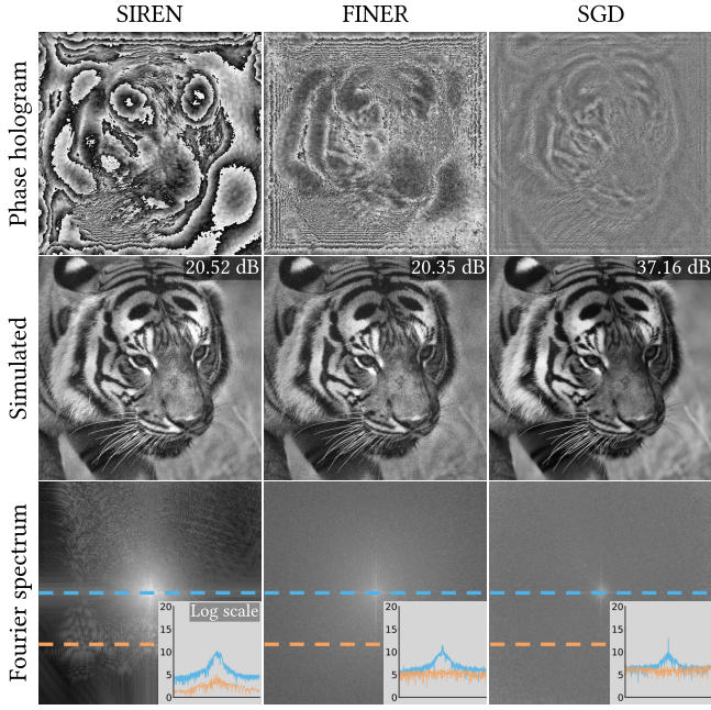
Fig. 3: Comparison of simulation results for studied INR-based (SIREN and FINER) and iterative (e.g., SGD) CGH methods. From top to bottom: phase holograms, reconstructed amplitudes, and corresponding magnitudes of the Fourier spectrum (log scale). FINER and SGD maintain broader spectral coverage and energy in high-frequency regions, while SIREN shows low-frequency components and exhibits sparse high-frequency activation. Dashed plots at the bottom indicate representative regions sampled to visualize the spectral distribution.
